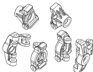
500406043 Achsschenkel-Set v+h Steering knuckle set, front & rear
