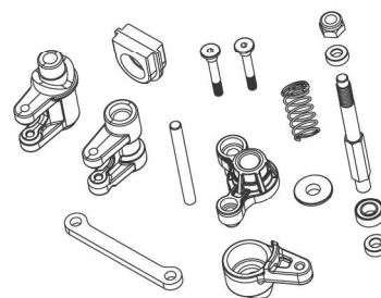
500406040 Servosaver/Lenkhebel-Set Servo saver / steering arm set
