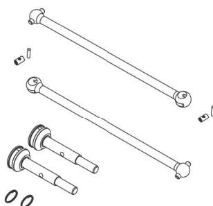
500406053 Kardangelenkwellen (2) vorne Front driveshafts (2)
